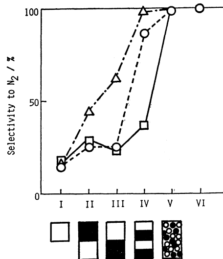
Fig. 4. Effect of the degree of mixing on the selectivity to \text{N}_2 in the oxidation of \text{NH}_3 with \text{MnO}_2 - \text{Pt}/\text{Al}_2\text{O}_3 .
